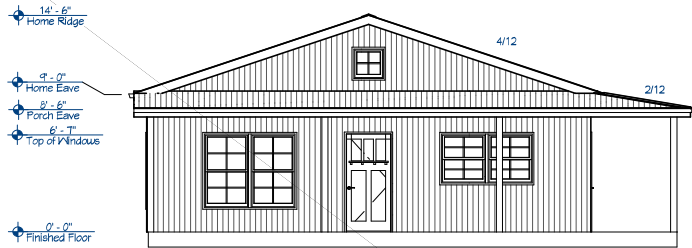
Exterior Elevation 1
